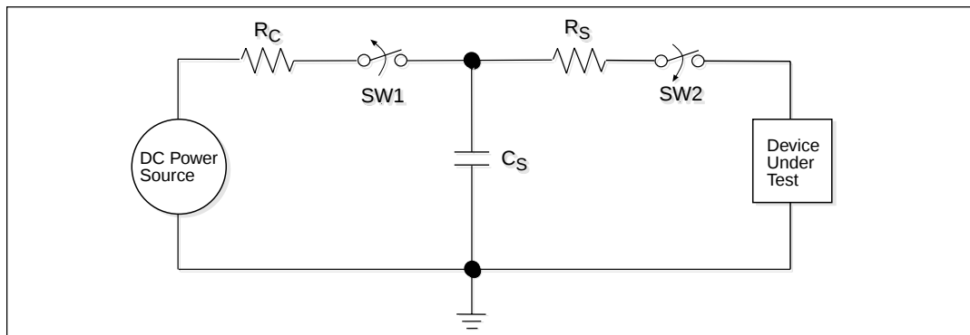
Figure 18. ESD Test Circuit for Human Body Model
