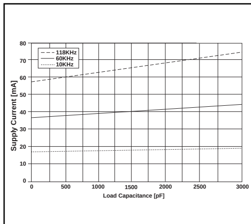
Figure 6. Supply Current VS. Load Capacitance when Transmitting Data for the SP3243EH
