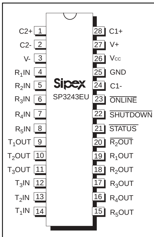
Figure 12. SP3243EU Pinout Configuration
