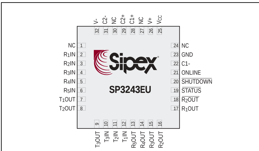
Figure 13. SP3243EU MLPQ Pinout Configuration
