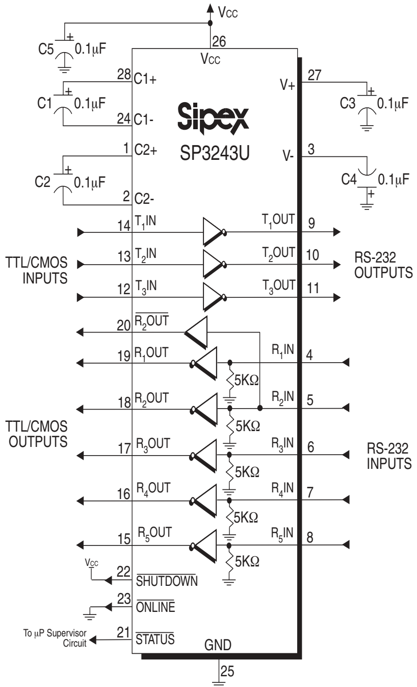
Figure 15. SP3243U Typical Operating Circuit
