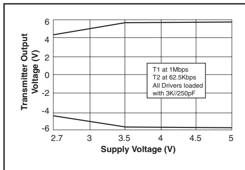
Figure 6. Transmitter Output Voltage VS. Supply Voltage for the SP3223U
