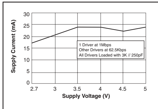
Figure 10. Supply Current VS. Supply Voltage for the SP3243U
