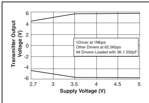
Figure 2. Transmitter Output Voltage VS. Supply Voltage for the SP3223U
