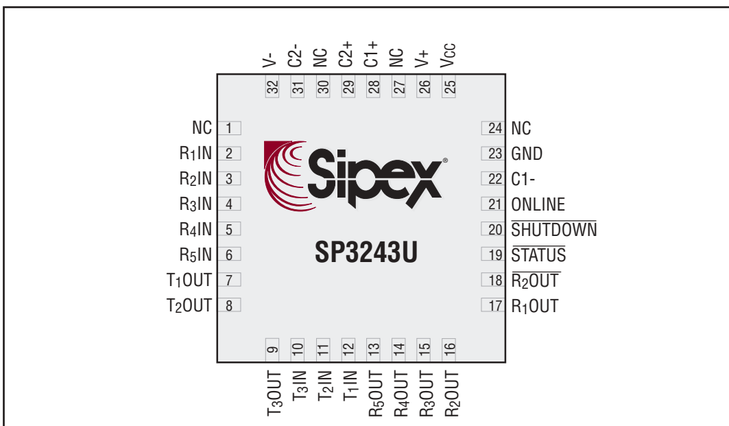
Figure 13. SP3243U QFN Pinout Configuration
