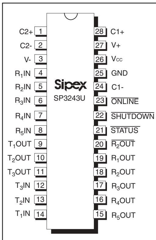
Figure 12. SP3243U Pinout Configuration
