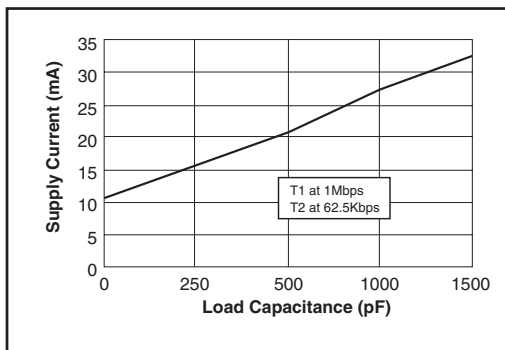
Figure 4. Supply Current VS. Load Capacitance for the SP3223U
