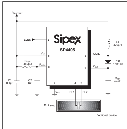
Figure 2. Typical Application Circuit for the SP4405, Set for a Square Wave Output with C_{\text{INT}} = 0.1\mu\text{F}
