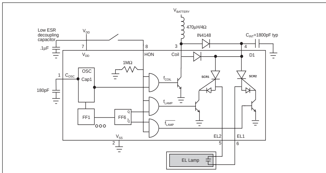
SP4425 Schematic
