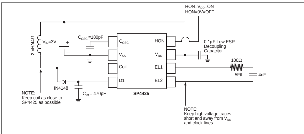
SP4425 3V Test Circuit
