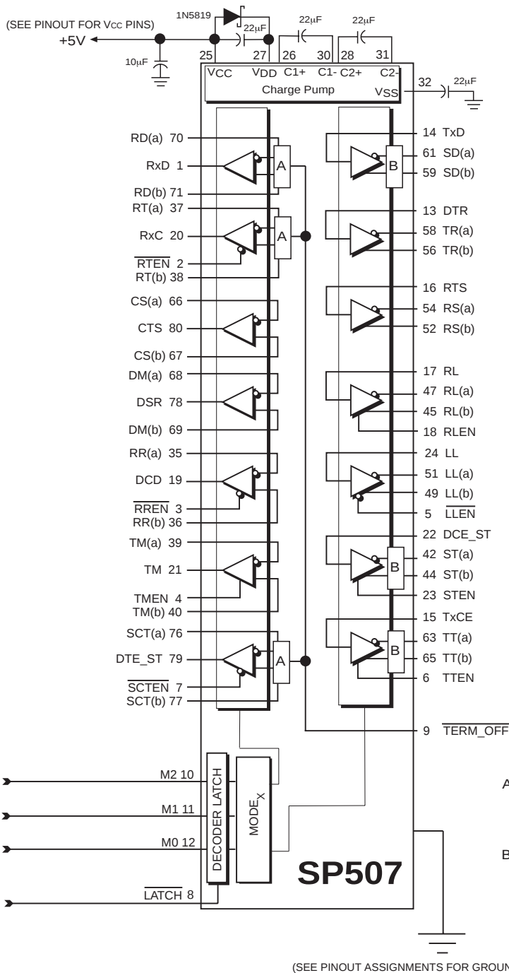
Figure 45. Typical Operating Circuit
