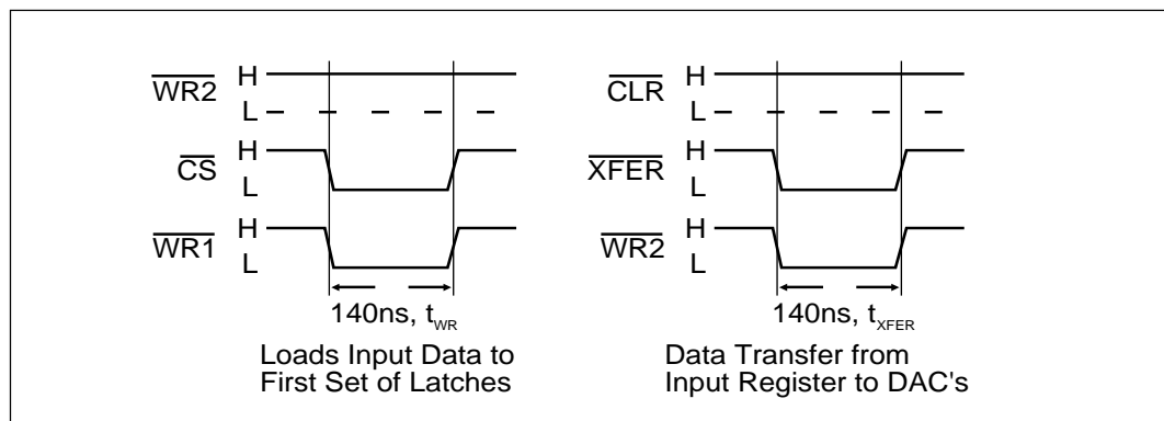
Figure 4. Timing
