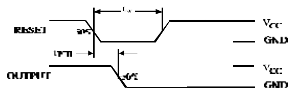
Figure 2. Switching Waveforms
