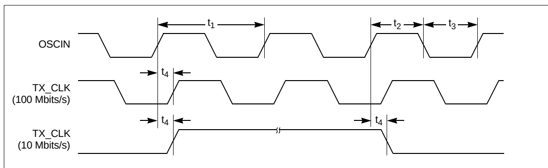
Figure 5.1 25 MHz Output Timing
