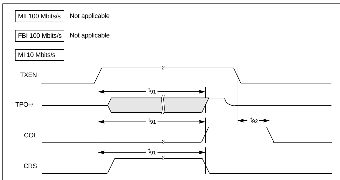
Figure 5.17 Jabber Timing
