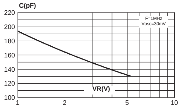
Fig. 4: Input capacitance versus reverse applied voltage (typical values).
