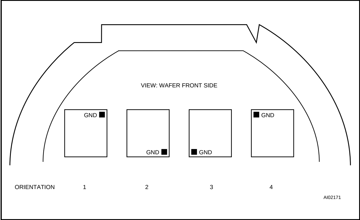
Figure 2. Sawing orientation
