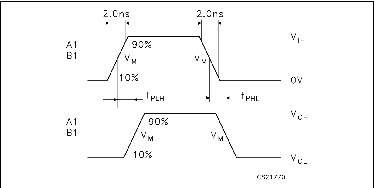
Figure 5: Waveform - Propagation Delay (f=1MHz; 50% duty cycle)
