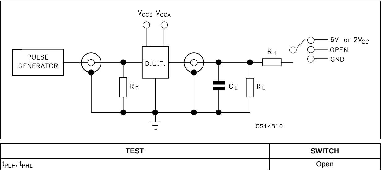
Figure 4: Test Circuit
