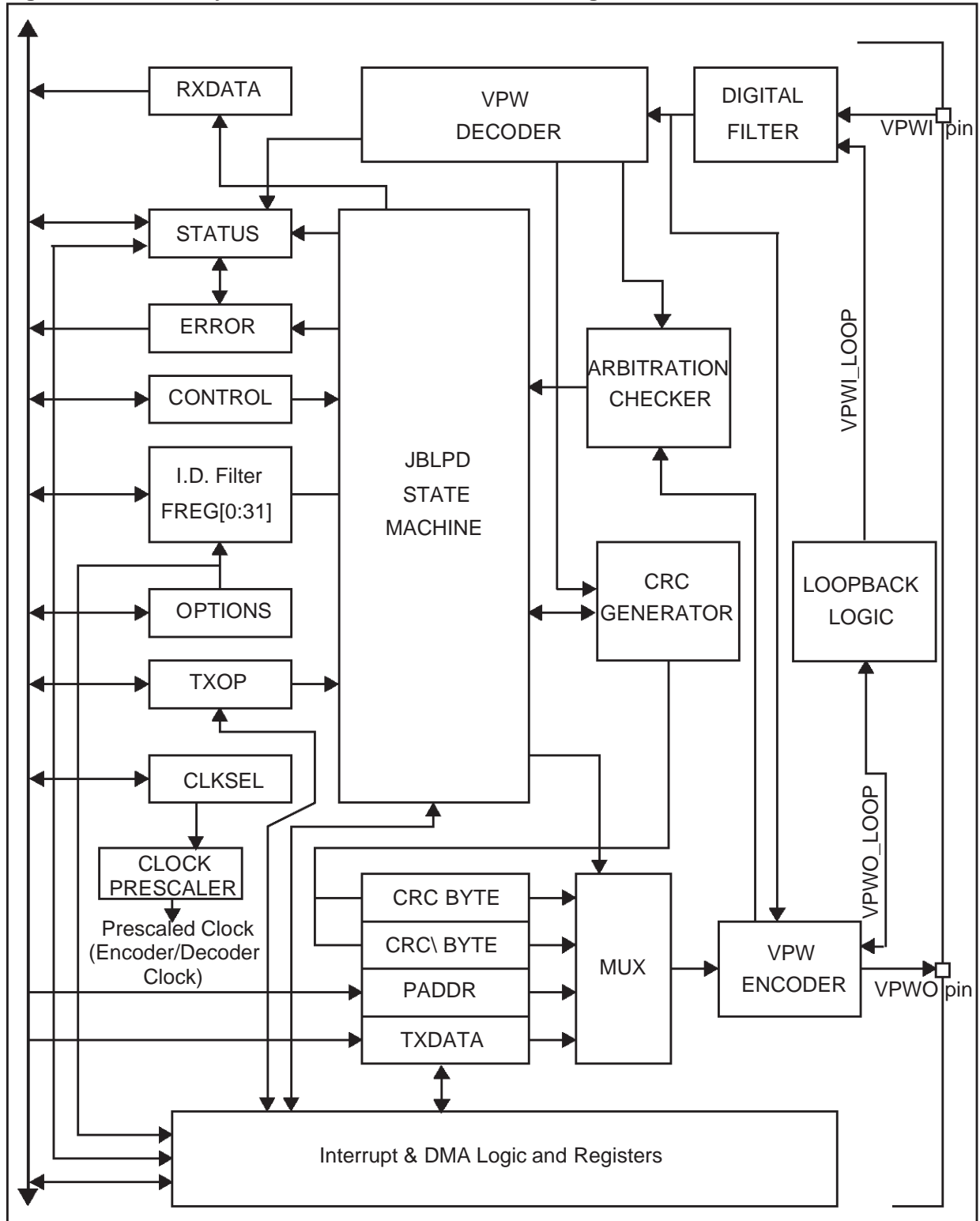
Figure 109. JBLPD Byte Level Protocol Decoder Block Diagram
