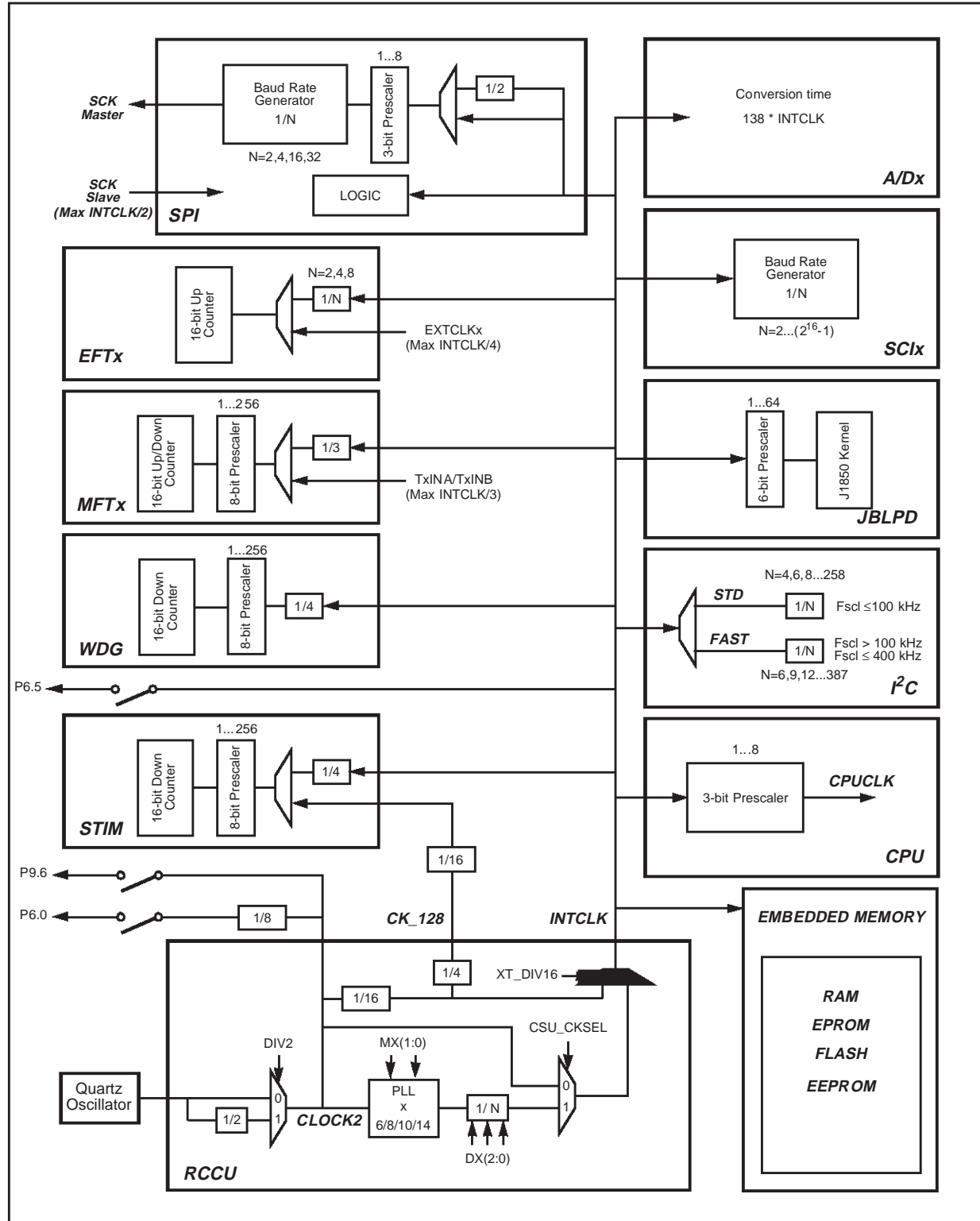
Figure 45. ST92F120 Clock Distribution Diagram
