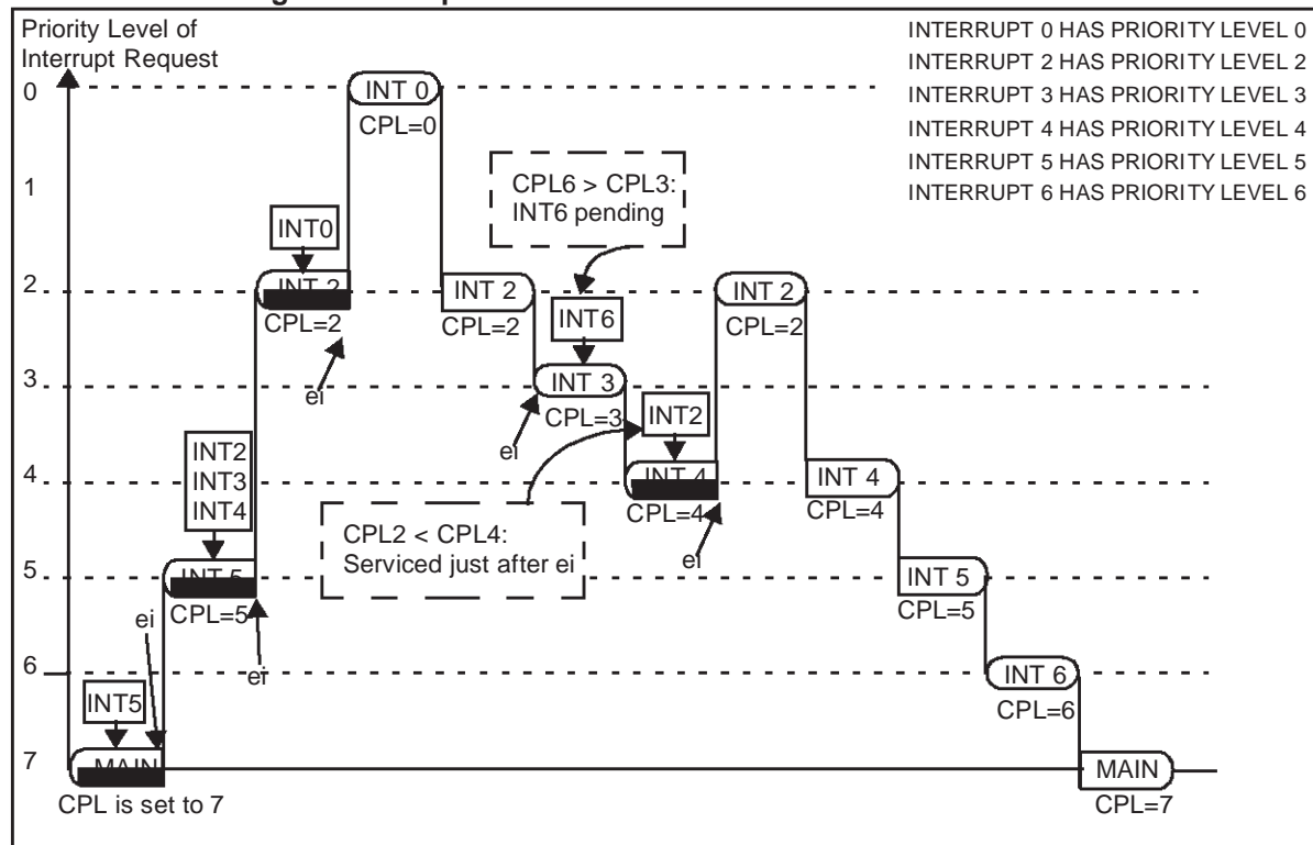
Figure 37. Complex Example of a Sequence of Interrupt Requests with:
