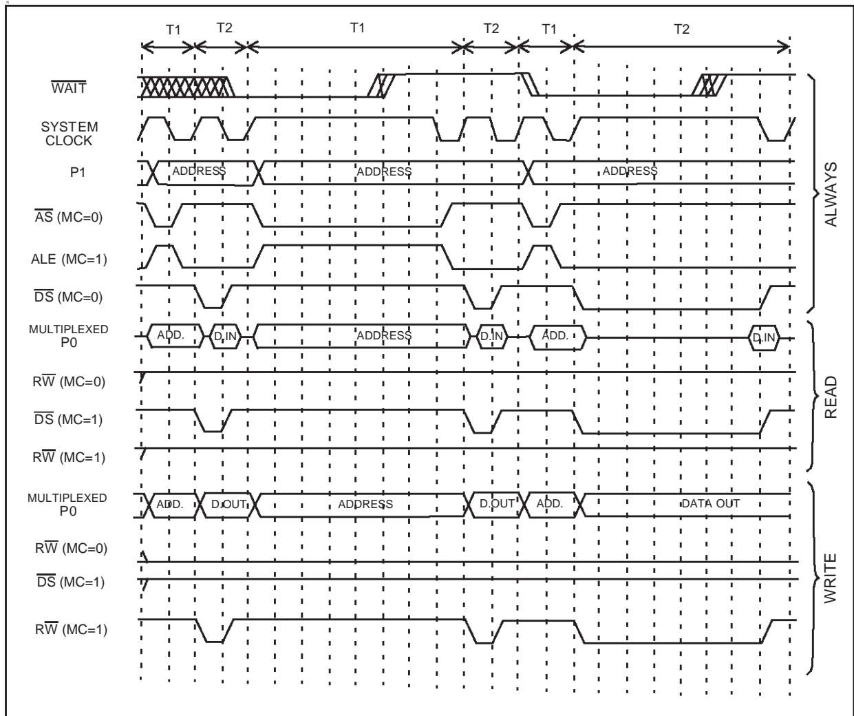
Figure 60. External memory Read/Write sequence with external wait ( \overline{WAIT} pin)
