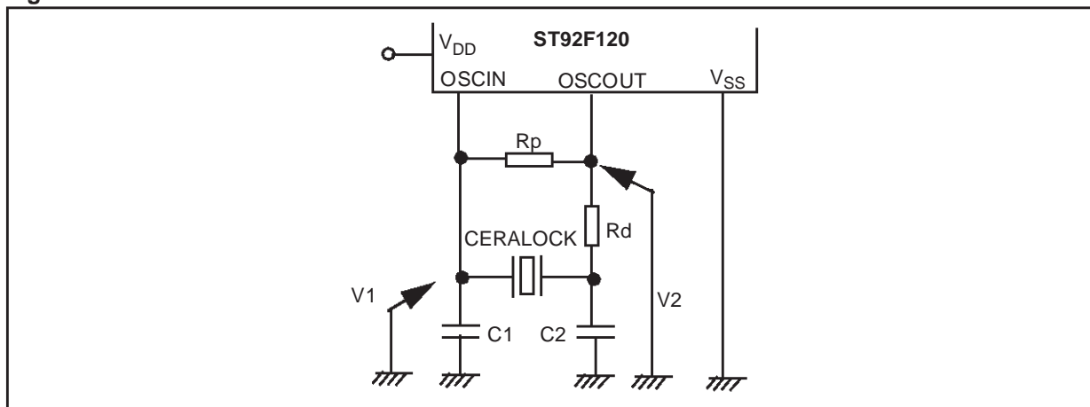
Figure 54. Test circuit
