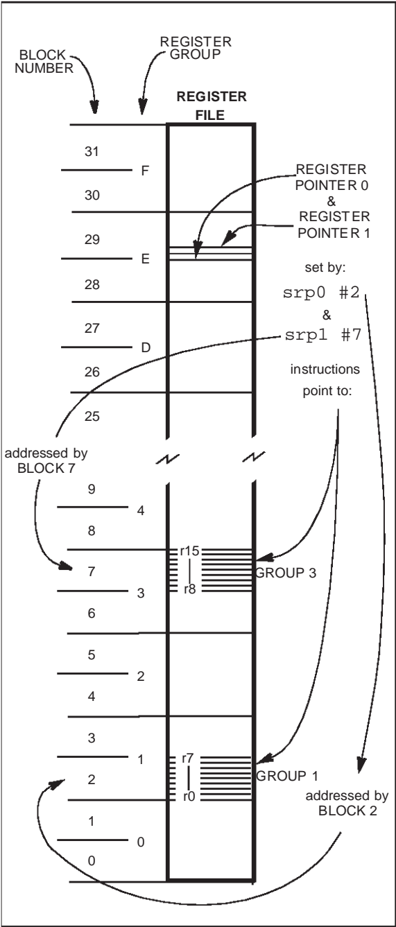
Figure 16. Pointing to two groups of 8 registers
