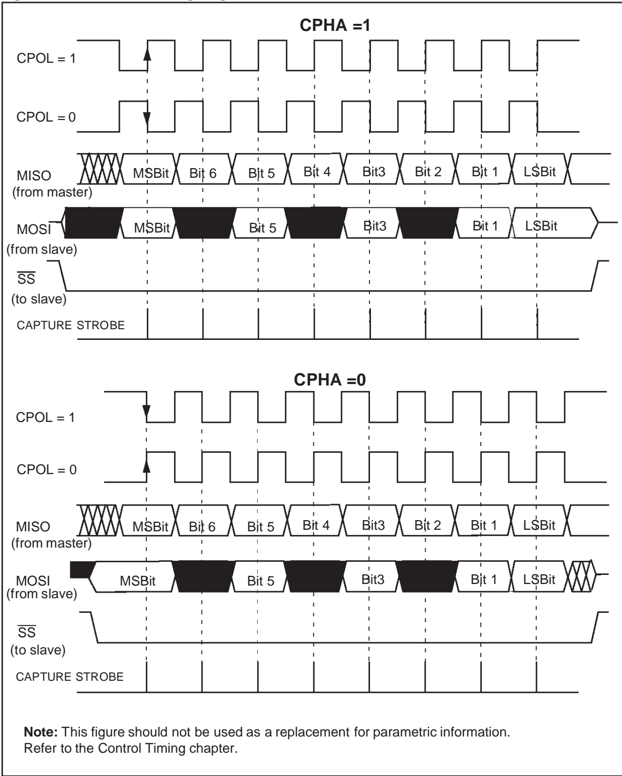
Figure 102. Data Clock Timing Diagram
