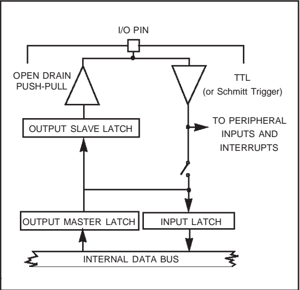
Figure 66. Output Configuration
