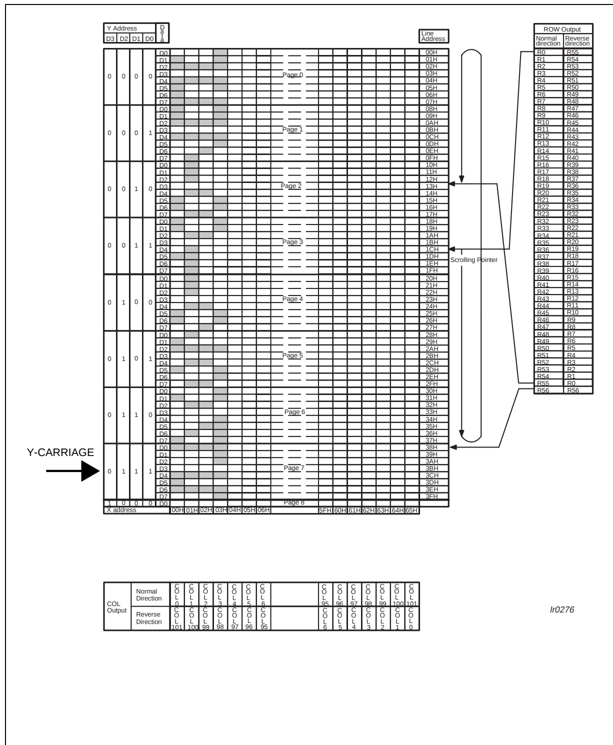
Figure 23. Memory Rows vs. Row Drivers Mapping ICON_MODE=1, Y-Carriage=7, Scrolling Pointer&gt;07h and MUX 49
