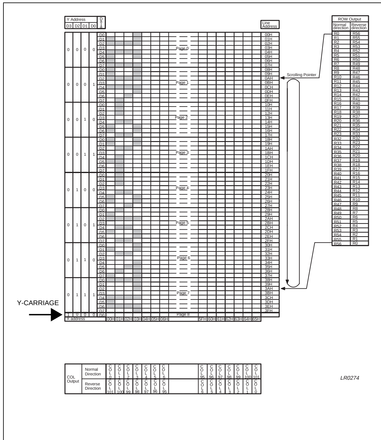
Figure 25. Memory Rows vs. Row Drivers Mapping ICON_MODE=0, Y-Carriage=8, Scrolling Pointer&lt;10h and MUX 49
