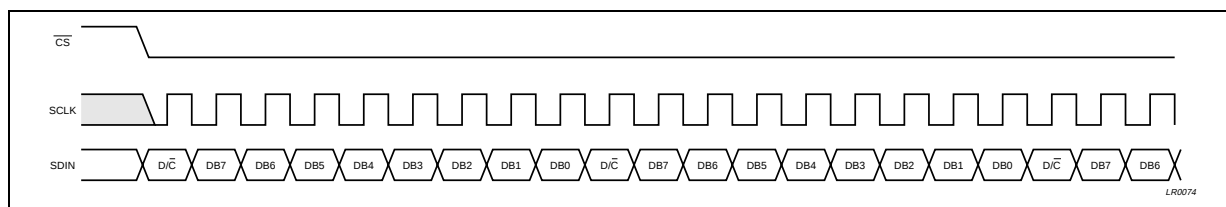
Figure 43. 3-lines serial interface protocol in Reading Mode
