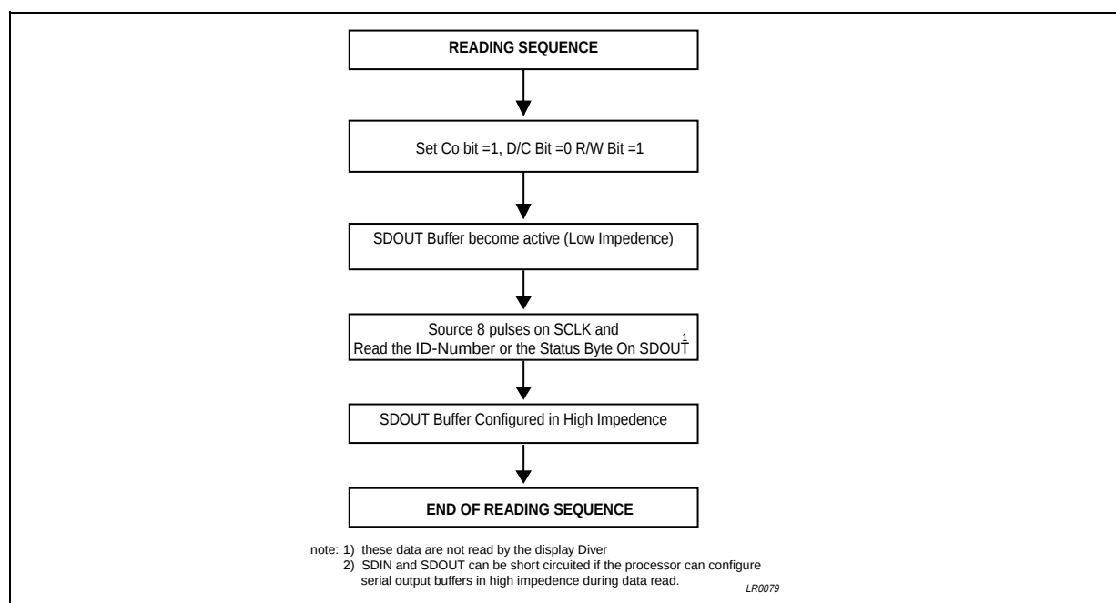
Figure 40. 3-lines SPI Reading Sequence
