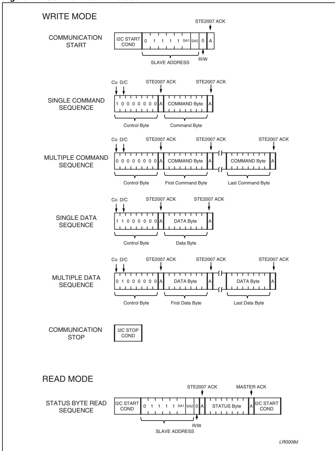
Figure 17. Communication Protocol
