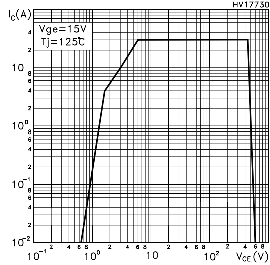
Turn-Off SOA
