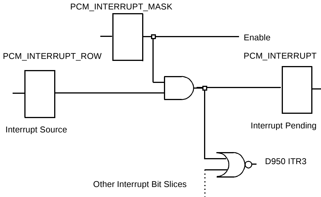
Figure 15: Interrupt Block
