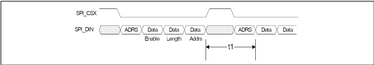
Figure 15. 3-WireShiftWait1
