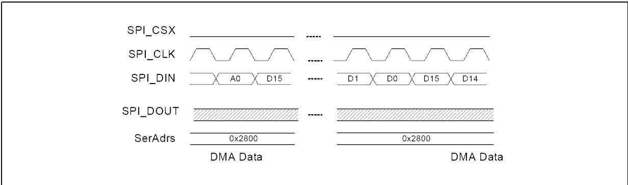
Figure 16. 3-WireInvShftWait1
