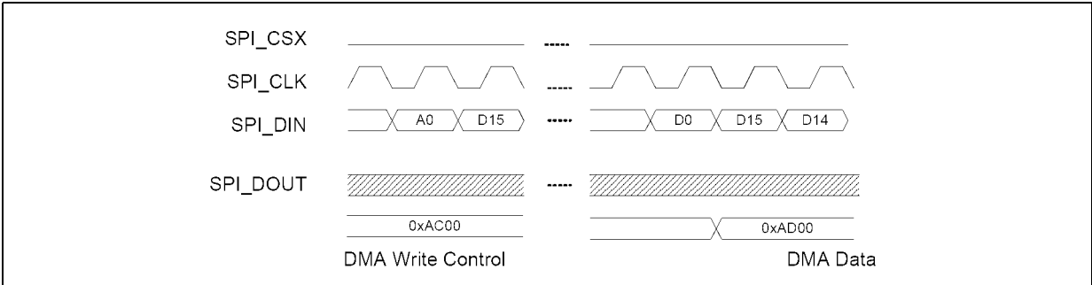
Figure 16. 3-WireInvShftWait1
