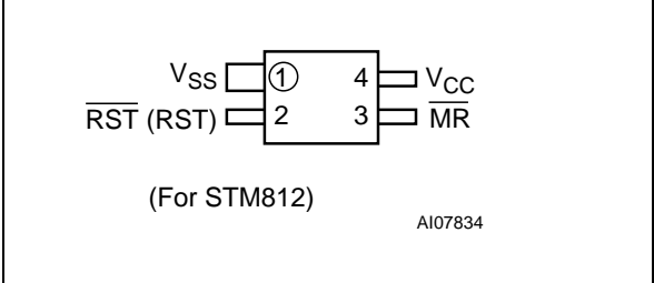
Figure 5. SOT143-4 Connections
