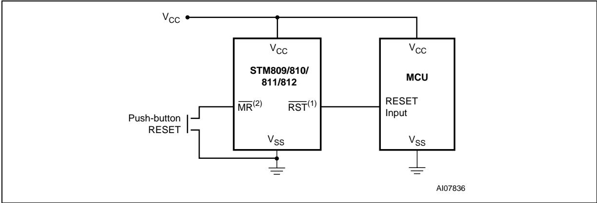
Figure 7. Hardware Hookup
