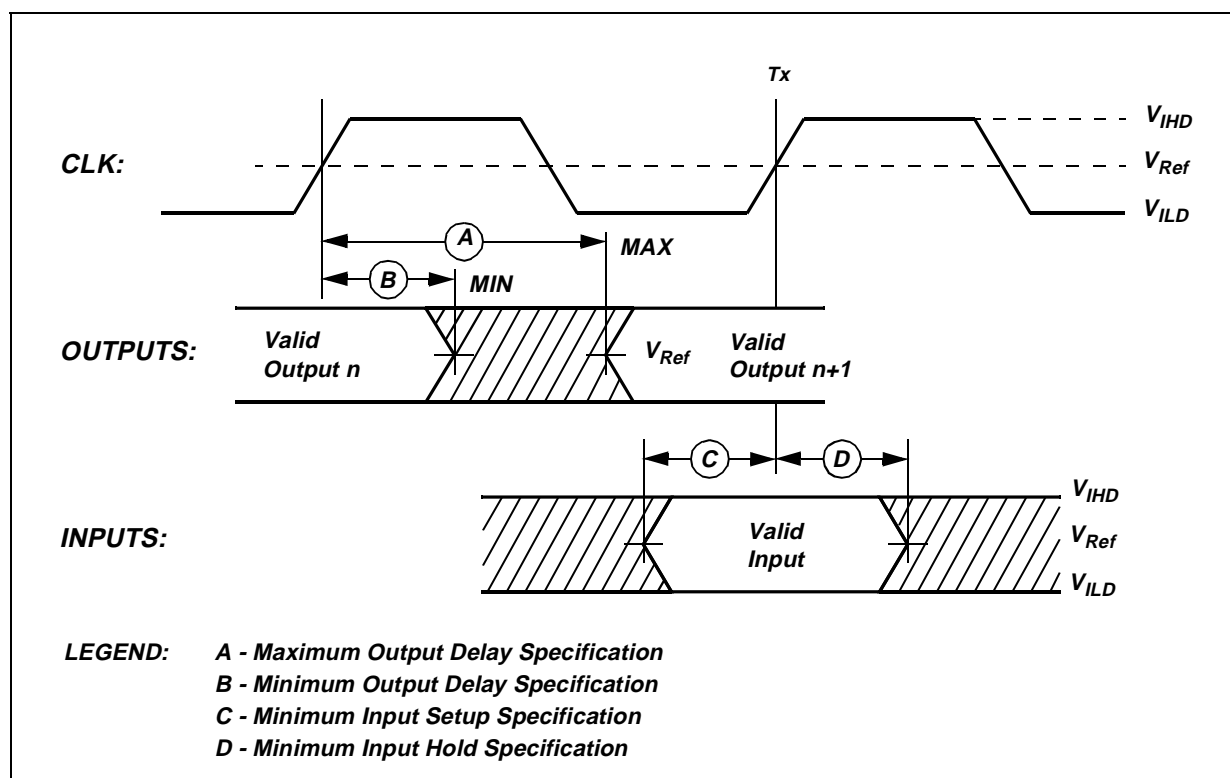
Figure 4-2 CLK Timing Measurement Points
