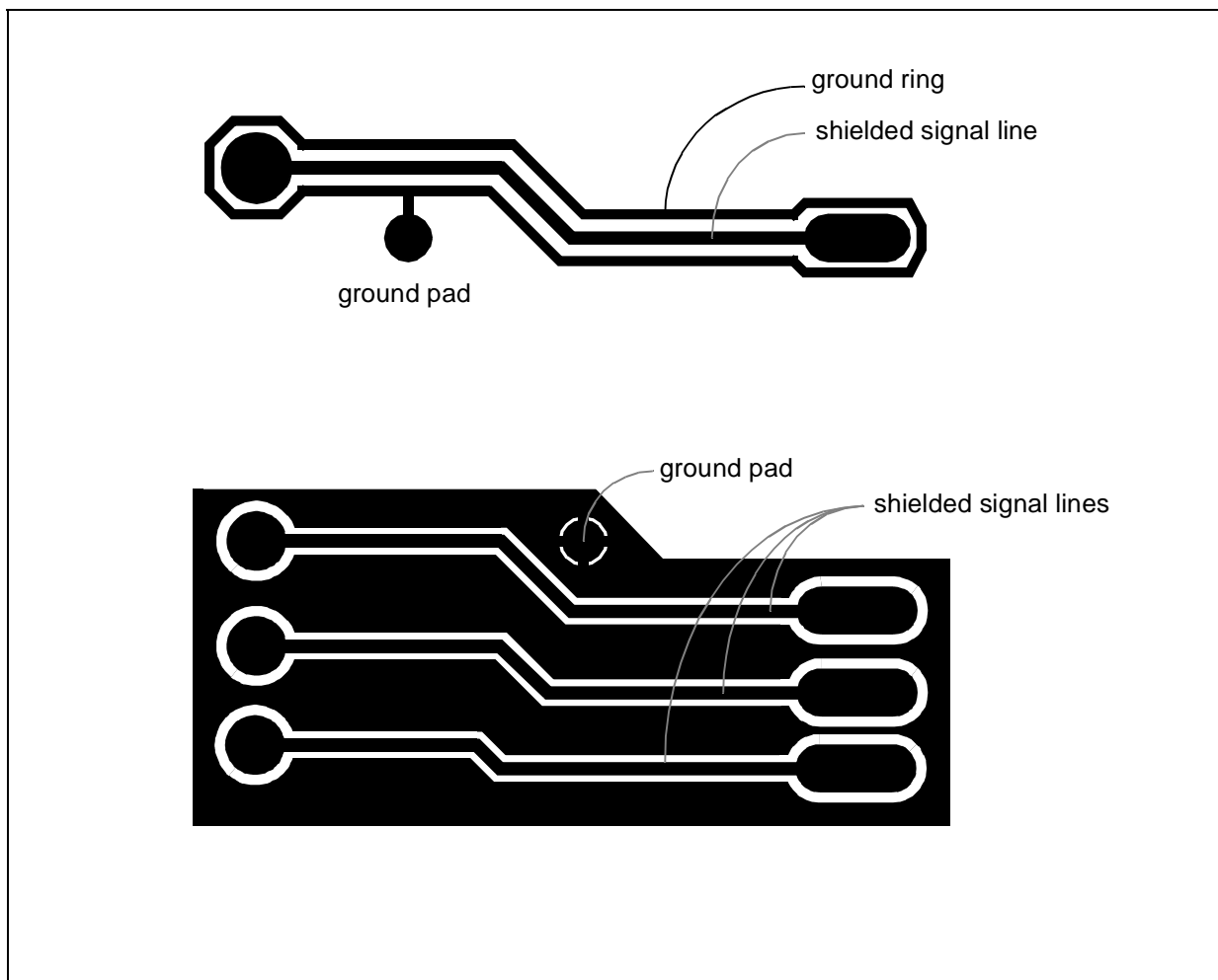
Figure 6-8. Shielding signals
