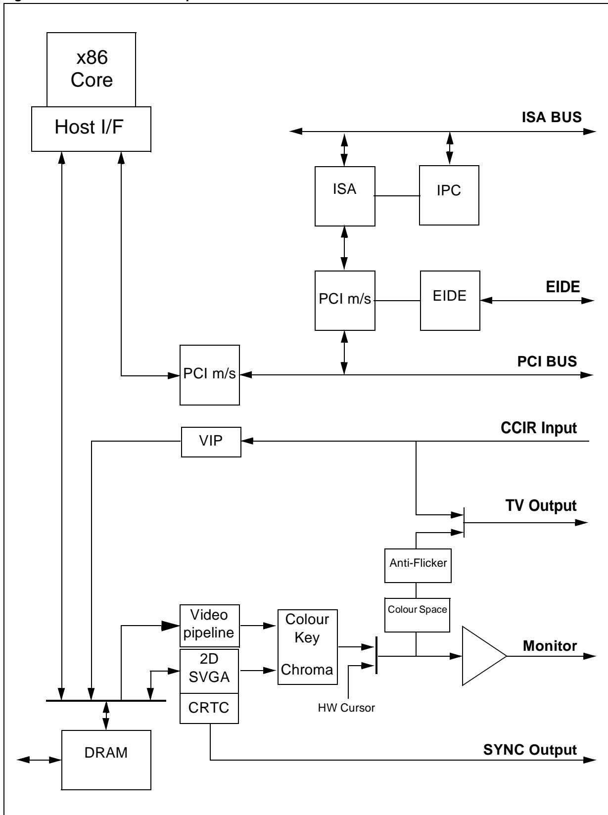
Figure 1-1. Functional description.
