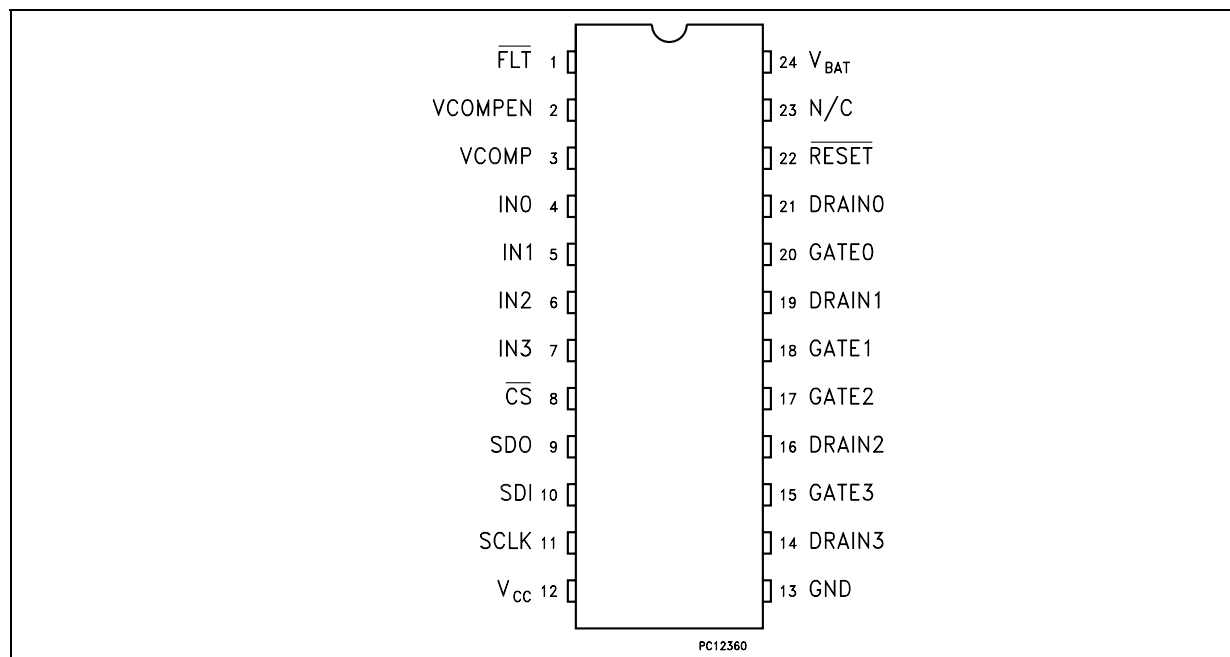
Figure 2 : Pin Configuration
