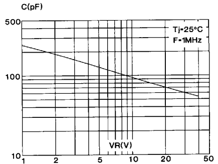
Fig. 9 : Junction capacitance versus reverse voltage applied. (Typical values) (Per diode)
