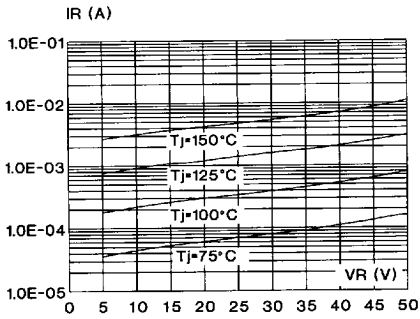
Fig. 8 : Reverse leakage current versus reverse voltage applied. (Typical values) (Per diode)
