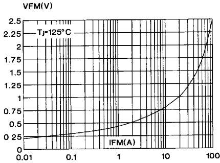
Fig. 10 : Forward voltage drop versus forward current. (Maximum values) (Per diode)
