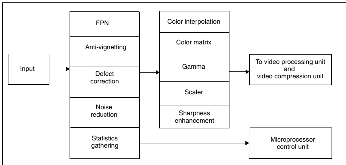
Figure 2: Video processing unit
