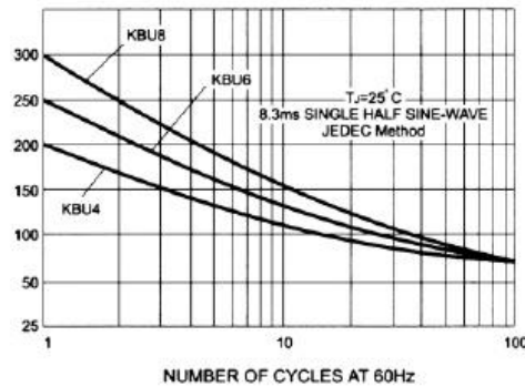
FIG. 3 - MAXIMUM NON-RETETITIVE PEAK FORWARD SURGE CURRENT
