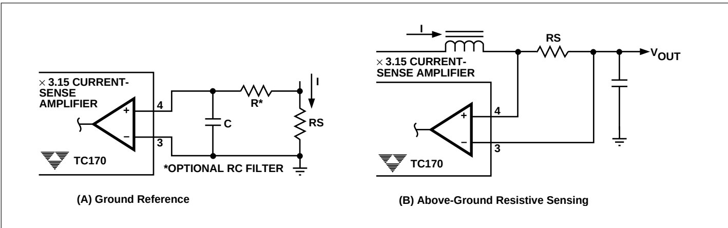
Figure 2. Resistive Sensing
