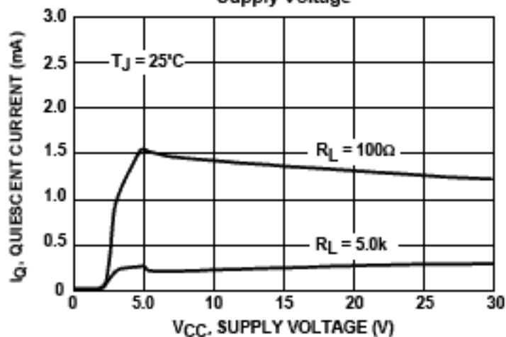
Figure 6. Quiescent Current versus Supply Voltage
