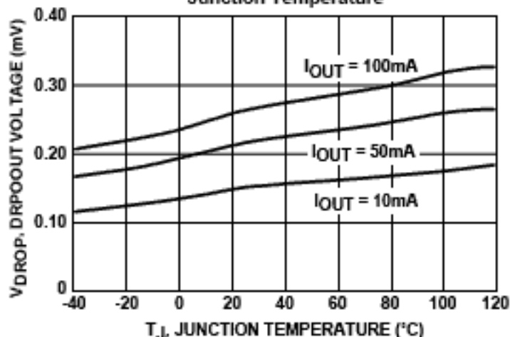
Figure 4. Dropout Voltage versus Junction Temperature
