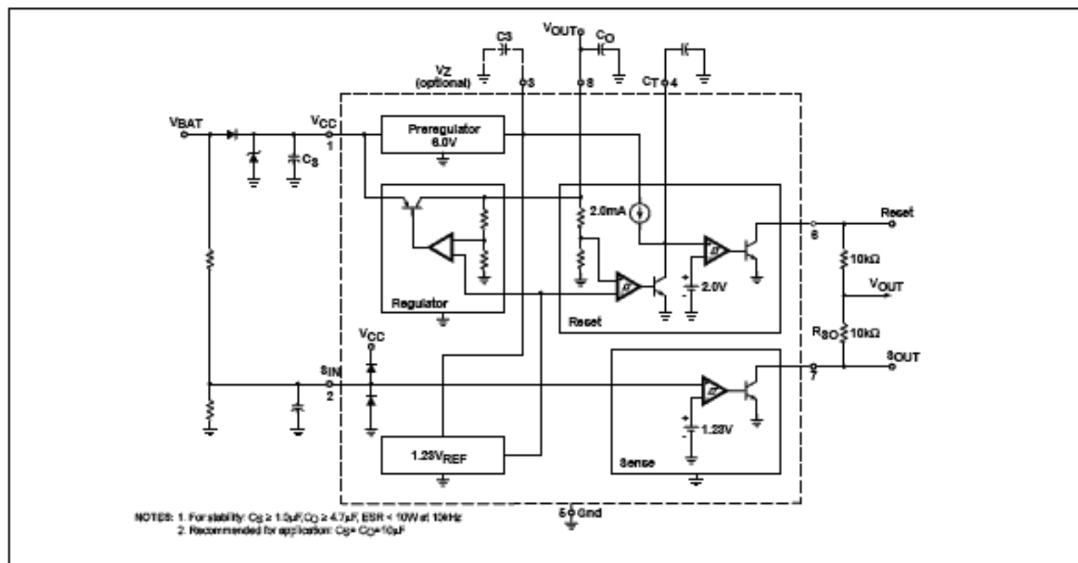
Figure 11. Application Schematic
