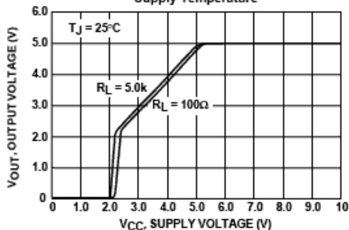
Figure 2. Output Voltage versus Supply Temperature
