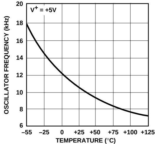
Unloaded Osc. Freq. vs. Temperature
