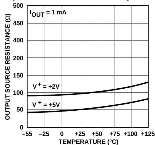
Output Source Resistance vs. Temperature
