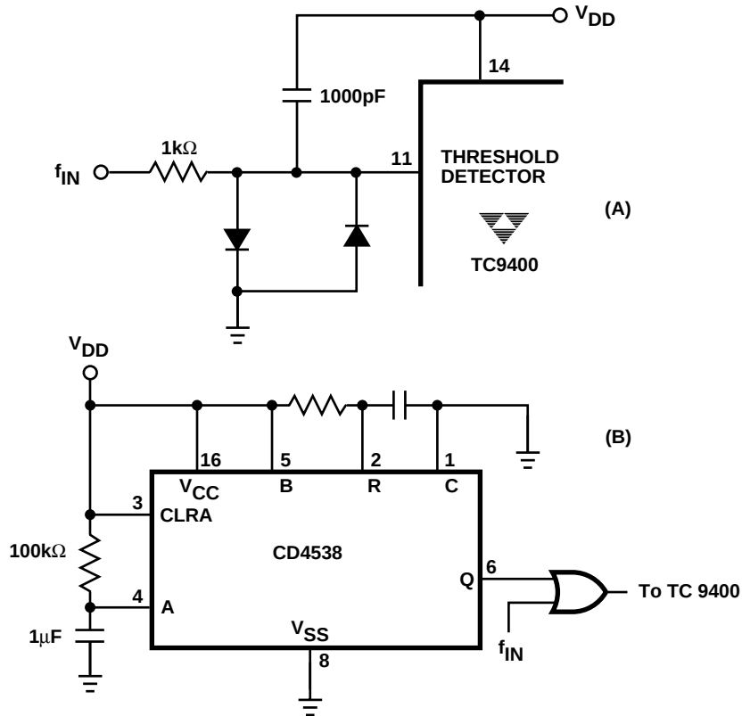
Figure 11. Power-On Operation/Reset
