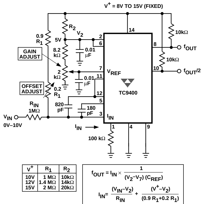
Figure 4 . Fixed Voltage — Single Supply Operation
