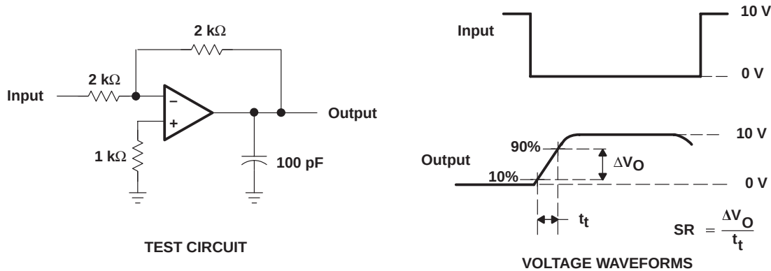
Figure 1. Slew Rate
