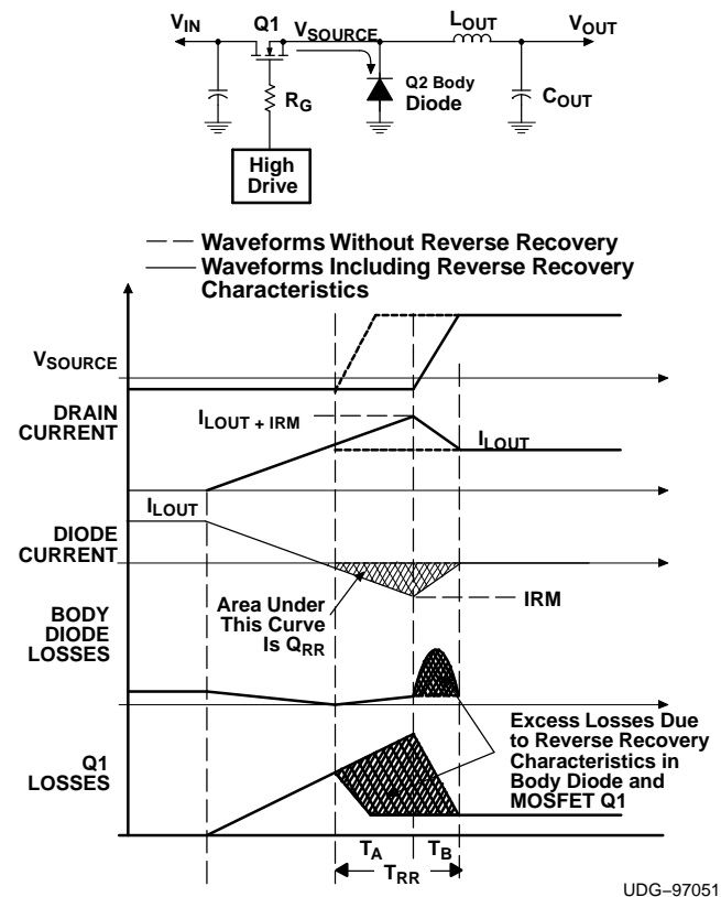
Figure 4. Effects of Reverse Recovery in a Synchronous Rectifier
