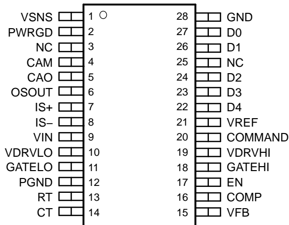
N, DW or PW PACKAGES (TOP VIEW)
