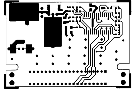
Figure 12. COMP Side
