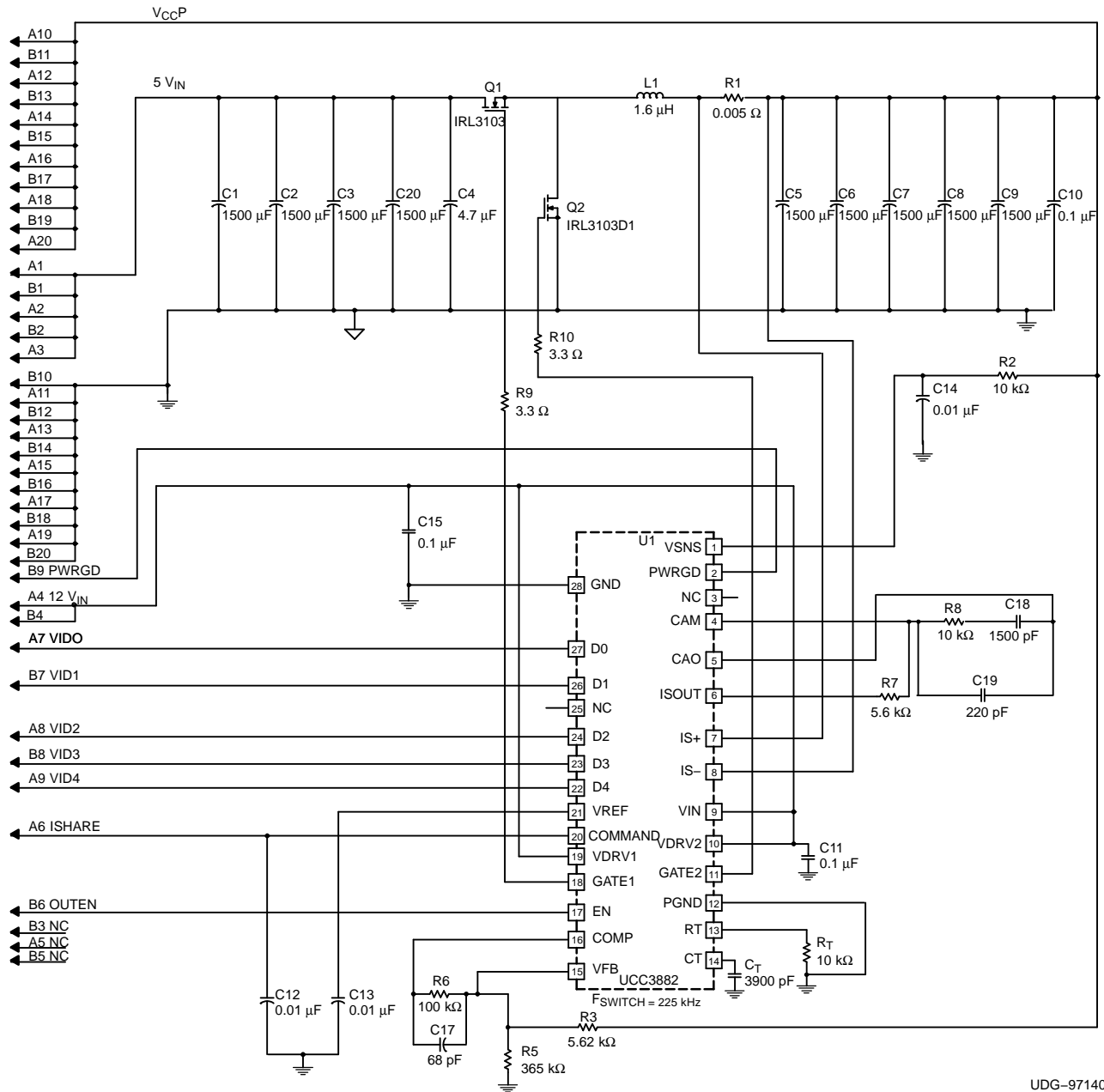
Figure 9. Reference Design – UCC3882 5-Bit Synchronous Wectifier PWM Controller for the Intel Pentium®II Processor
