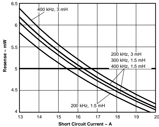
Figure 5. Short Circuit Current Limit vs R_{SENSE} for Various Frequency and Inductor Values
