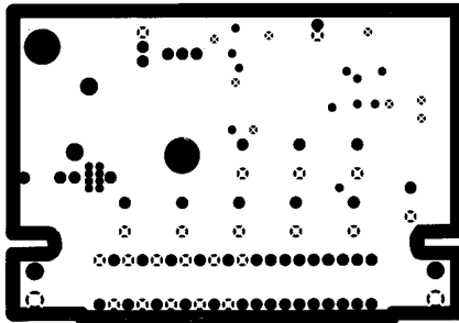
Figure 13. GND Layer
