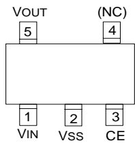
SOT-25 (SOT-23-5) (TOP VIEW)
