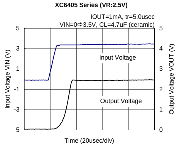
(17) Rising Response Time (Continued)
