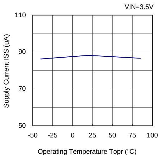
XC6405 Series (VR:2.5V)
