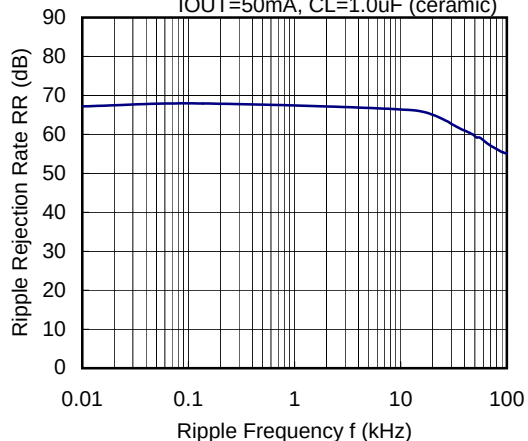
XC6405 Series (VR:2.5V)
