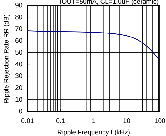
XC6405 Series (VR:3.0V)
