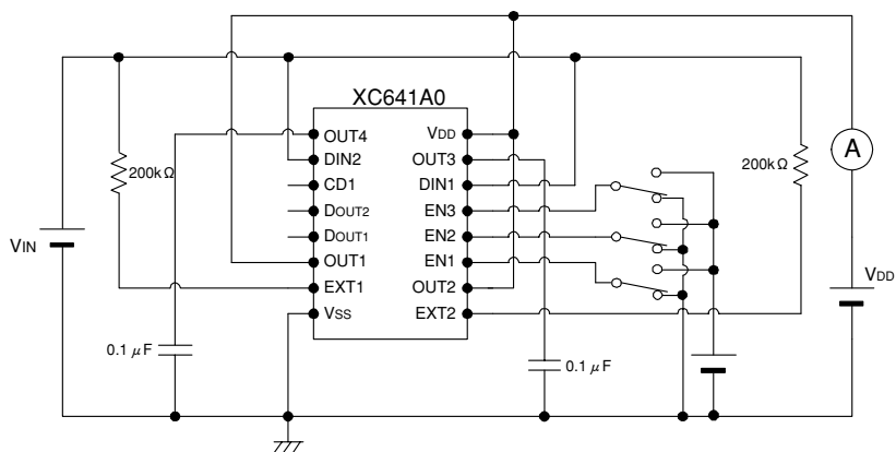
Application Circuit 2
