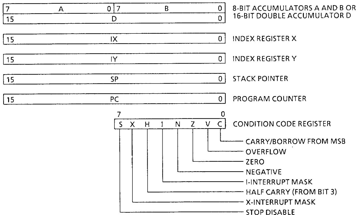
Figure 1.2 Programming Model
