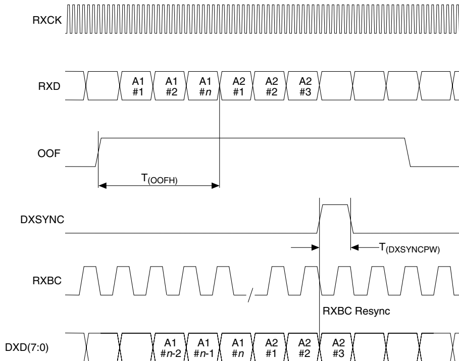
Figure 8. Demultiplexer Timing
