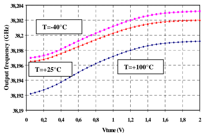
Typical tuning characteristic
