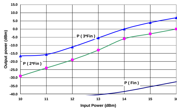
Pout versus Pin @ Fin=14GHz &amp; Vd=4V
