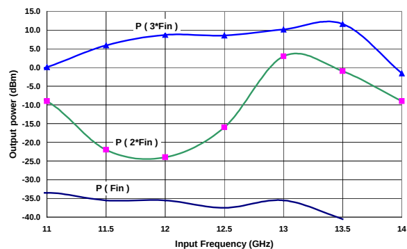
Pout versus Fin @ Pin=14 dBm &amp; Vd=3.5V
