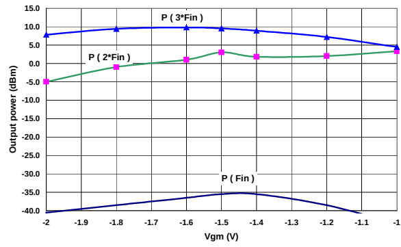
Pout versus Vgm @ Fin=13GHz &amp; Vd=3V
