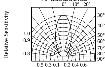
FIG.6 SENSITIVITY DIAGRAM
