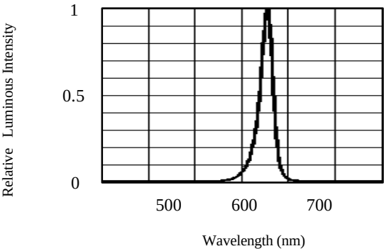
FIG.1 RELATIVE LUMIINOUS INTENSITY VS. WAVELENGTH
