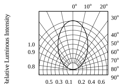
FIG.6 RADIATION DIAGRAM
