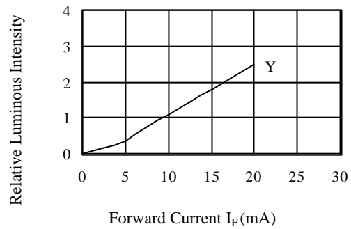
FIG.2-1 RELATIVE LUMINOUS INTENSITY VS. FORWARD CURRENT
