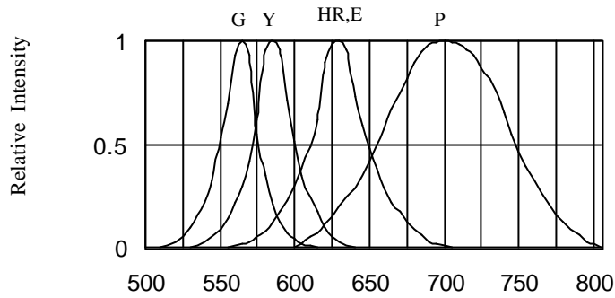
FIG.1 RELATIVE LUMINOUS INTENSITY VS. WAVELENGTH
