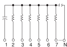
Circuit E
