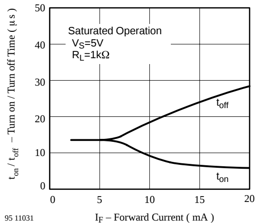
95 11031 Figure 12. Turn on / off Time vs. Forward Current
