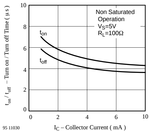
95 11030 Figure 13. Turn on / off Time vs. Collector Current
