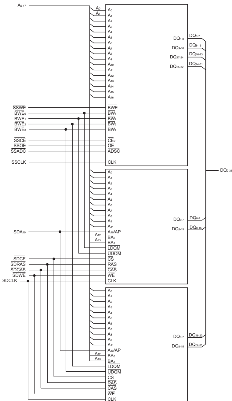
FIG. 2 BLOCK DIAGRAM
