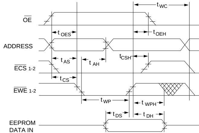
FIG. 7 EEPROM WRITE WAVEFORMS \overline{\text{EWE}} CONTROLLED
