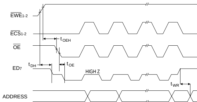
FIG. 10 EEPROM DATA POLLING WAVEFORMS
