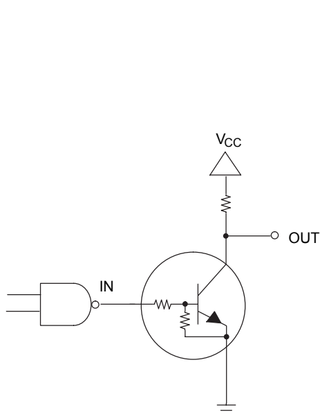
Figure 29. Open Collector Inverter: Inverts the Input Signal
