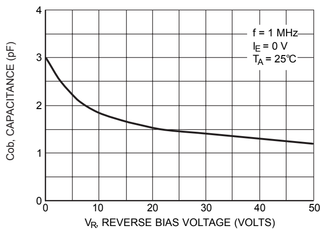
Figure 15. Output Capacitance
