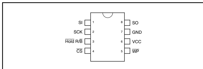
Figure 3A. NX25F011B and NX25F021B Pin Assignments, 8-Pin SOIC
