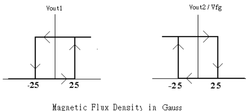
WSH411 Complementary Output1 vs.Output2/Vfg
