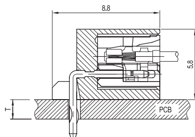
PCB ASSY
